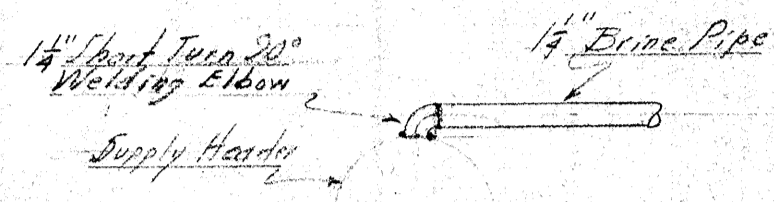
TYPICAL CONNECTION SUPPLY HEADER Scale - 1" = 1'-0"
