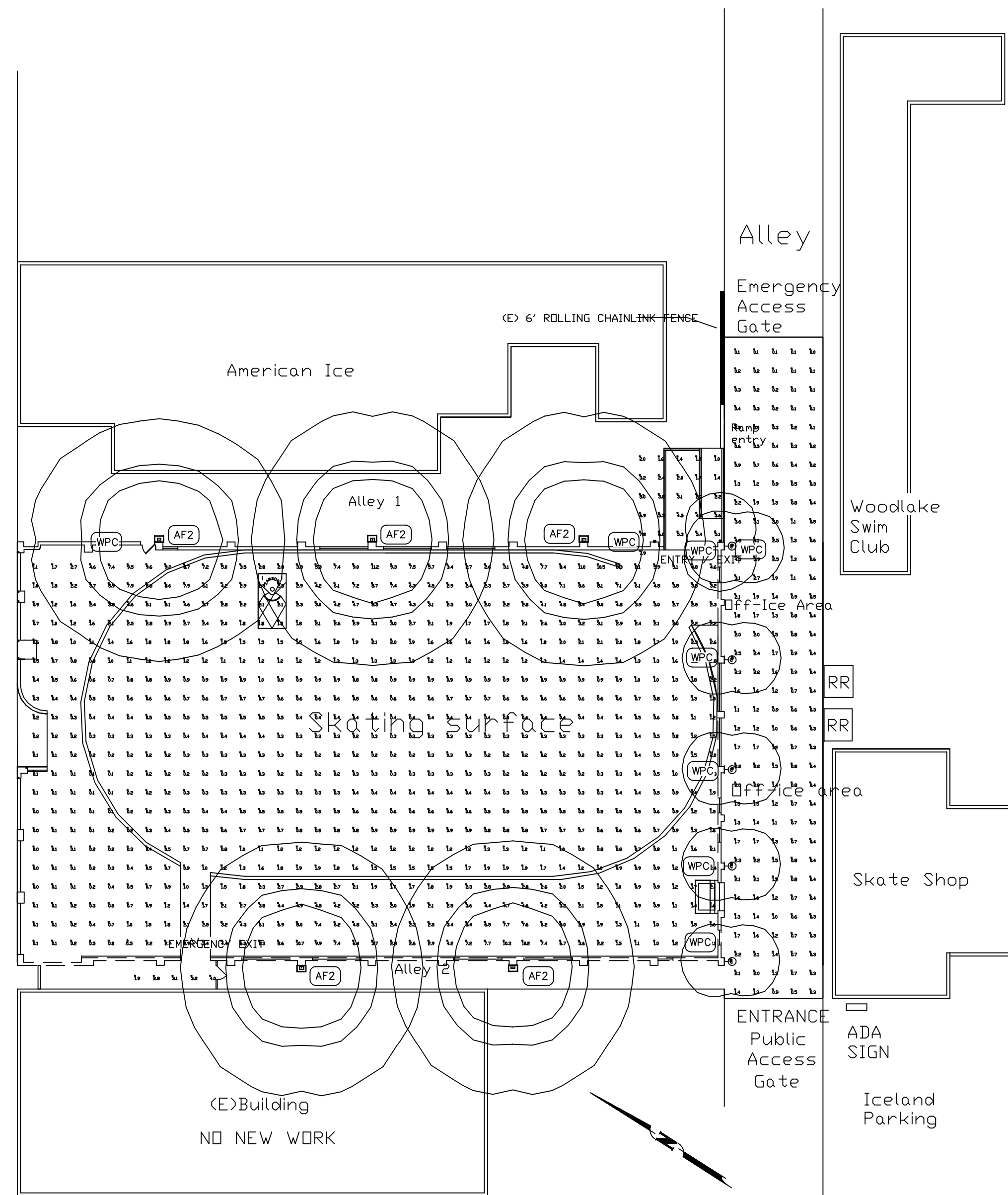
E2.2 ELECTRICAL SITE PLAN- PHOTOMETRICS SCALE: 1/16" = 1'-0" FEBRUARY 03, 2011
